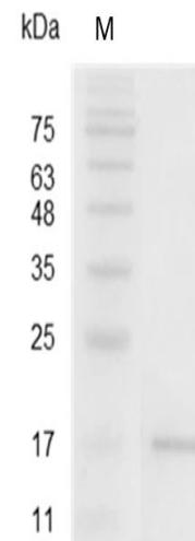
SDS-PAGE analysis of recombinant mouse LIGHT
